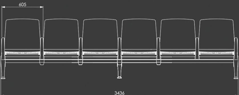
VIVA MULTISEATER - 6 SEATER WEIGHT - 43.37 KG
