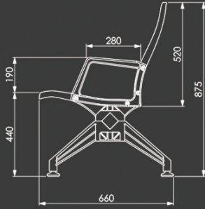
VIVA MULTISEATER - 1 SEATER WEIGHT - 10.82 KG
