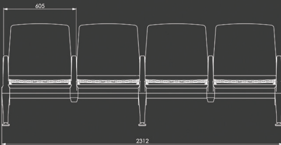
VIVA MULTISEATER - 4 SEATER WEIGHT - 30.72 KG
