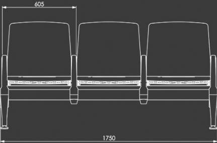
VIVA MULTISEATER - 3 SEATER WEIGHT - 23.72 KG
